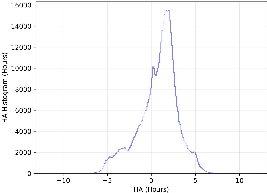
too_elab_r256_d2_gz_v3.4_10yrs WFD i band: HA Histogram
