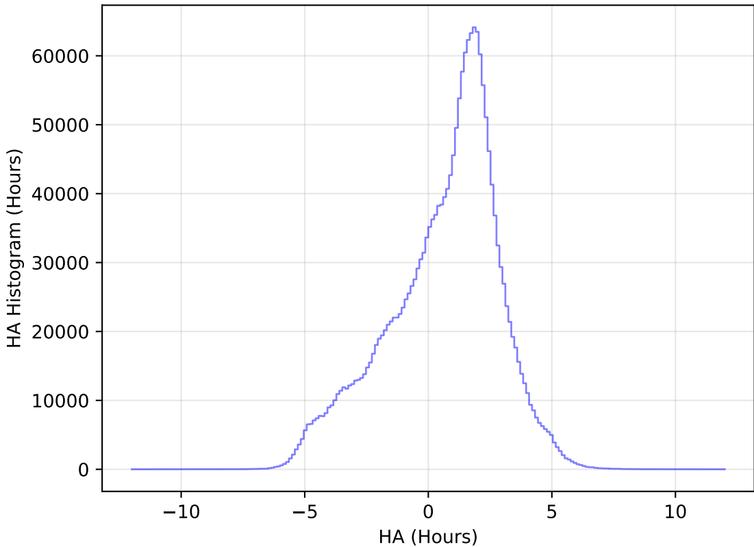
too_elab_r256_d2_gz_v3.4_10yrs WFD all bands: HA Histogram
