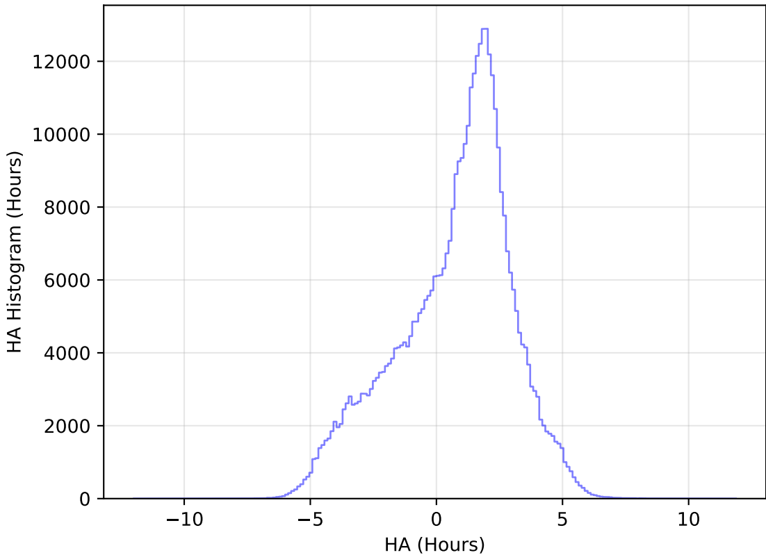
too_elab_r256_d2_gz_v3.4_10yrs All sky z band: HA Histogram
