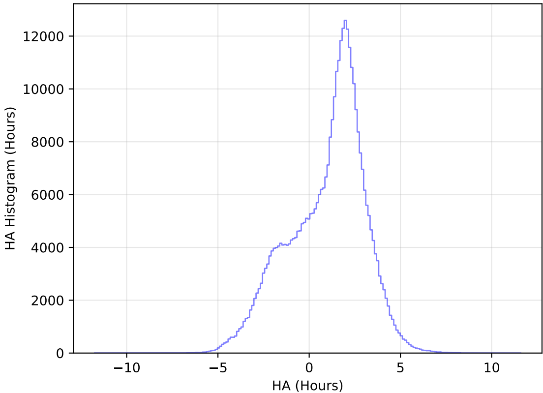
too_elab_r256_d2_gz_v3.4_10yrs All sky y band: HA Histogram
