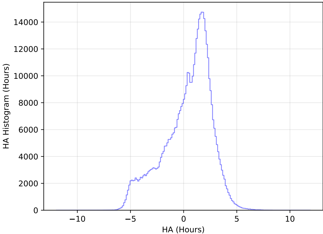
too_elab_r256_d2_gz_v3.4_10yrs All sky r band: HA Histogram
