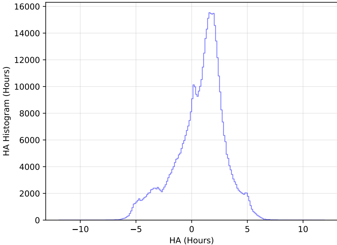
too_elab_r256_d2_gz_v3.4_10yrs All sky i band: HA Histogram
