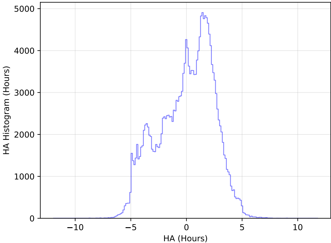
too_elab_r256_d2_gz_v3.4_10yrs All sky g band: HA Histogram
