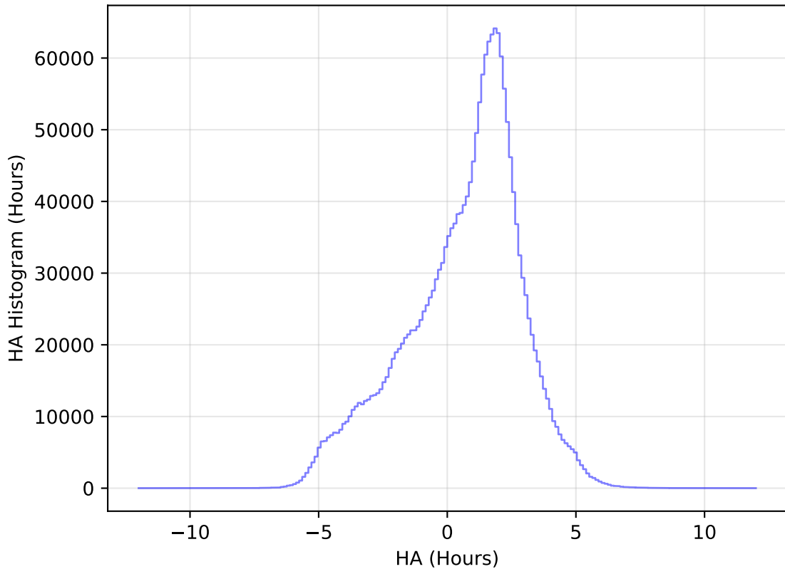
too_elab_r256_d2_gz_v3.4_10yrs All sky all bands: HA Histogram
