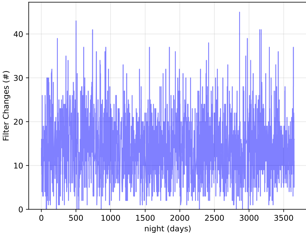
too_elab_r256_d2_gz_v3.4_10yrs Per Night: Filter Changes
