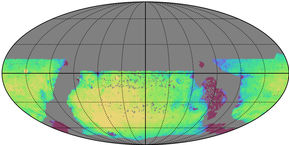
too_elab_r256_d2_gz_v3.4_10yrs WFD r band: Exgal_CoaddM5
