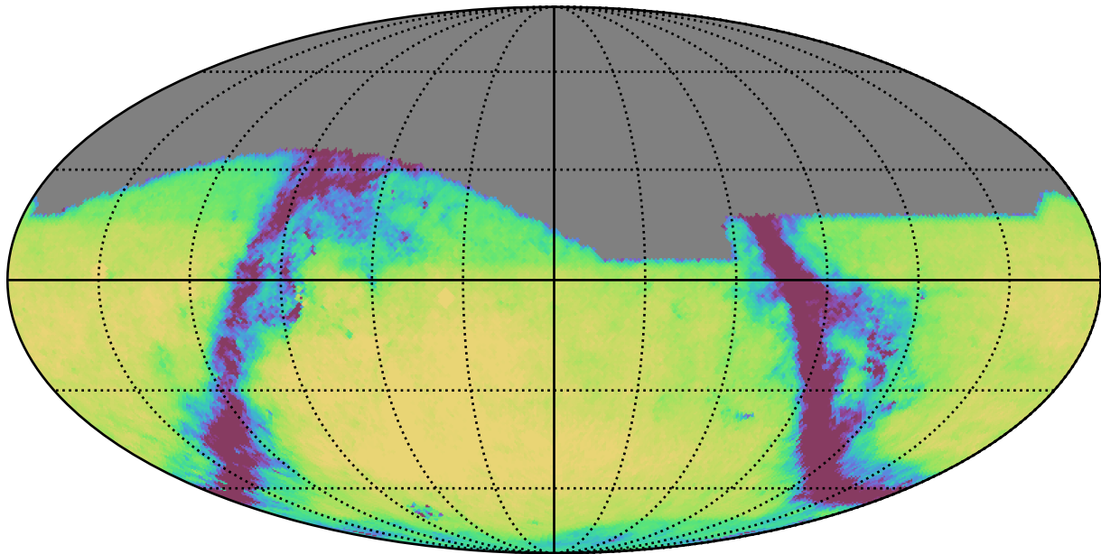
too_elab_r256_d2_gz_v3.4_10yrs All sky g band: Exgal_CoaddM5
