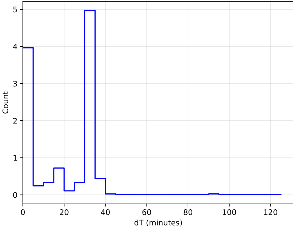
too_elab_r256_d2_gz_v3.4_10yrs WFD: DeltaT Histogram
