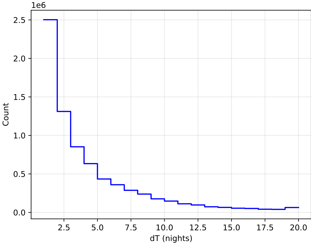
too_elab_r256_d2_gz_v3.4_10yrs WFD all bands: DeltaNight Histogram
