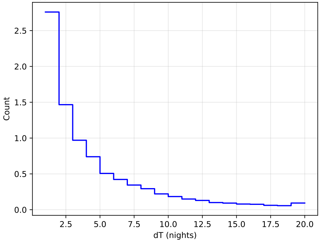
too_elab_r256_d2_gz_v3.4_10yrs All sky all bands: DeltaNight Histogram
