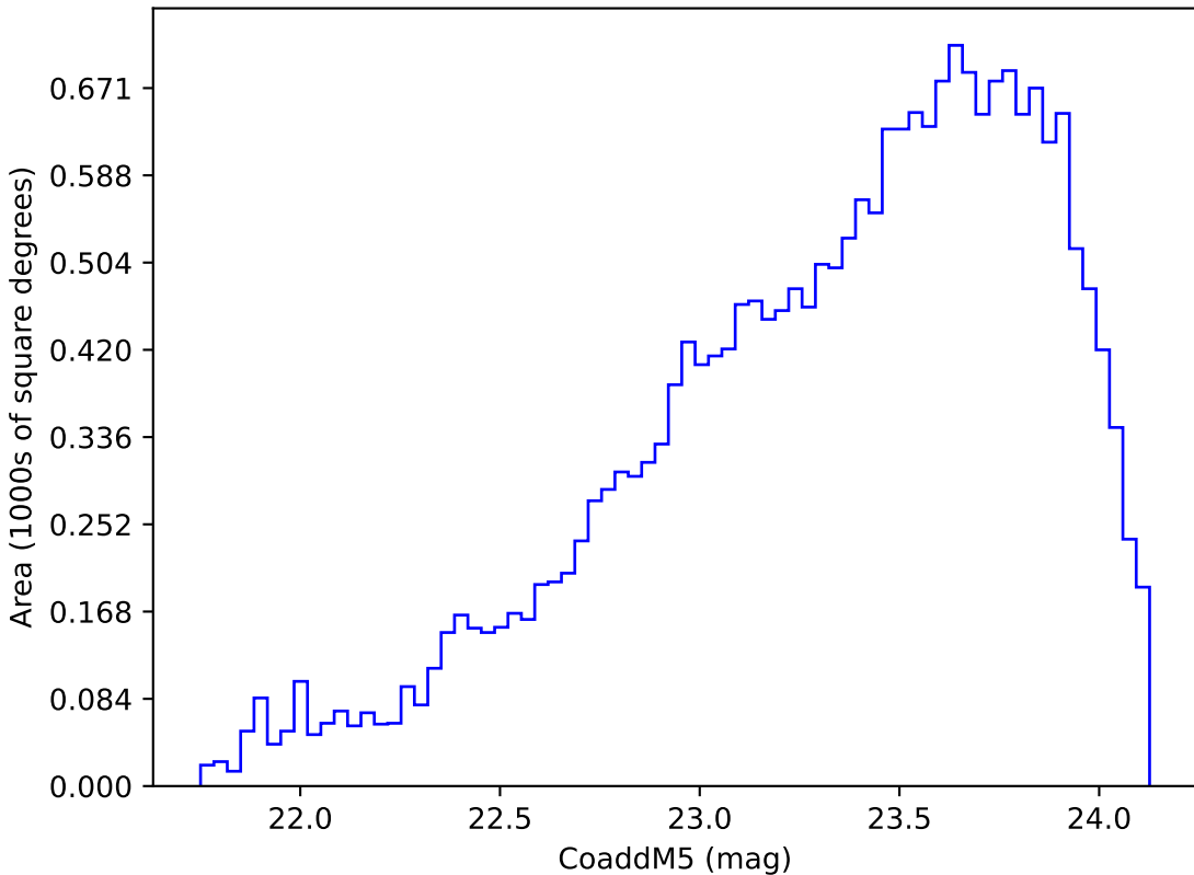
too_elab_r256_d2_gz_v3.4_10yrs Yr 3-4 y band: CoaddM5
