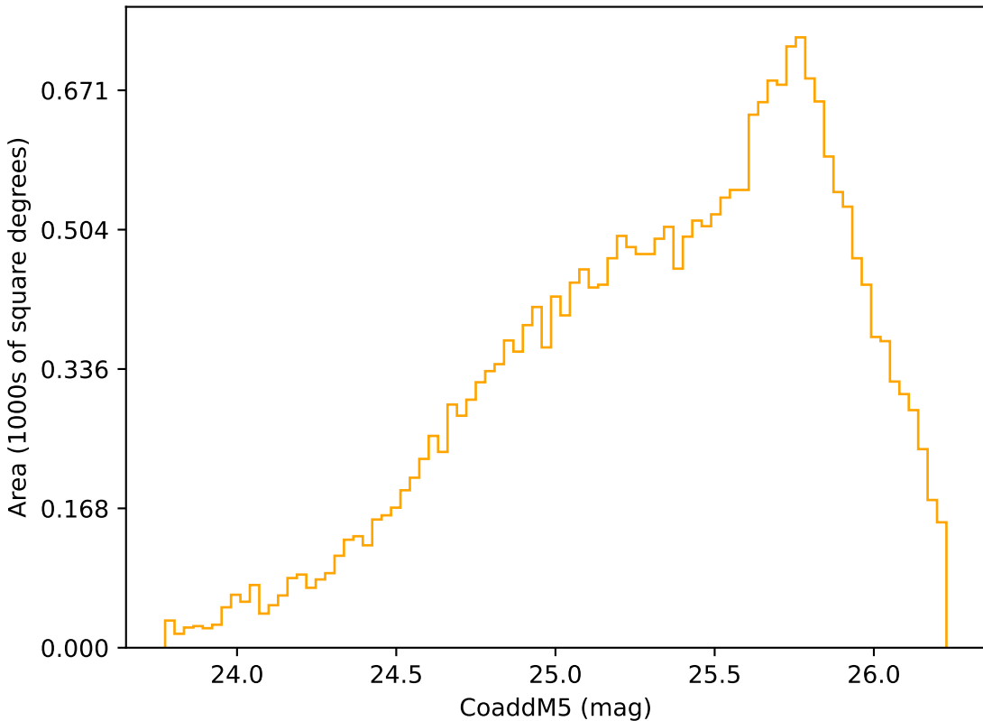
too_elab_r256_d2_gz_v3.4_10yrs Yr 3-4 r band: CoaddM5
