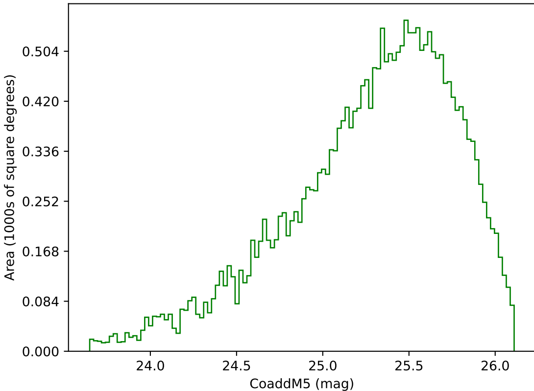
too_elab_r256_d2_gz_v3.4_10yrs Yr 3-4 g band: CoaddM5
