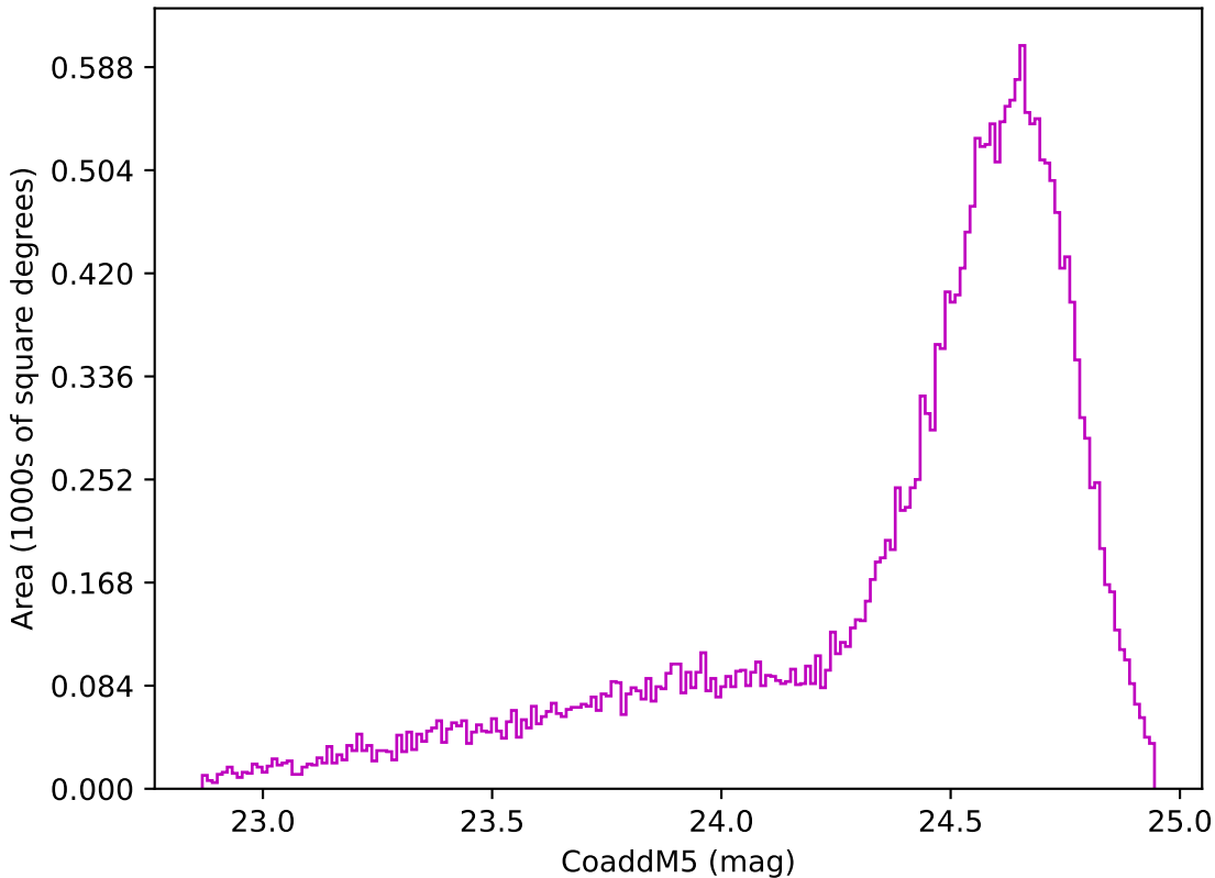
too_elab_r256_d2_gz_v3.4_10yrs Yr 1 z band: CoaddM5
