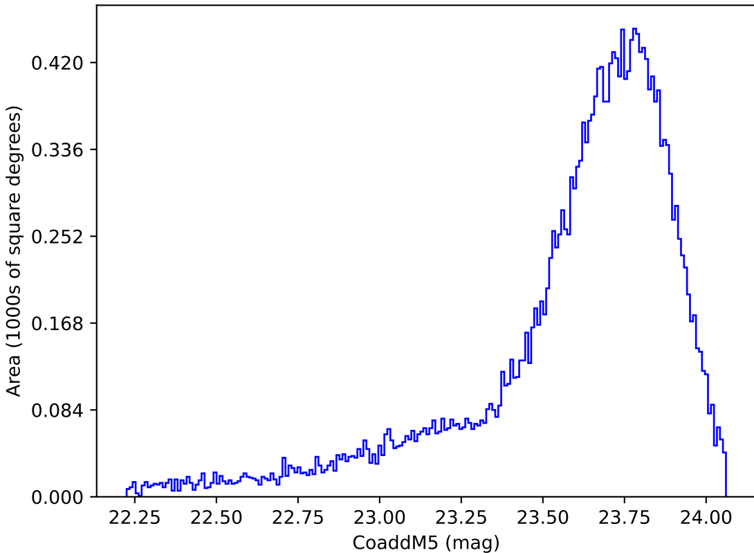
too_elab_r256_d2_gz_v3.4_10yrs Yr 1 y band: CoaddM5
