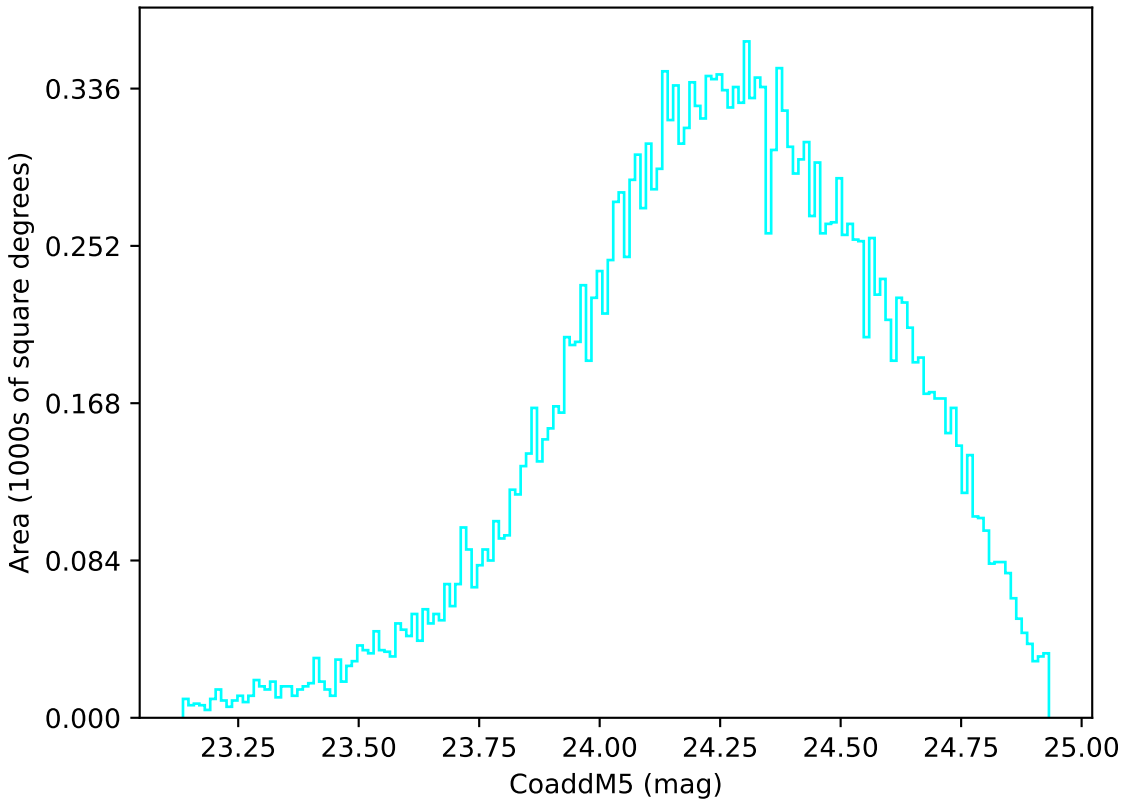
too_elab_r256_d2_gz_v3.4_10yrs Yr 1 u band: CoaddM5
