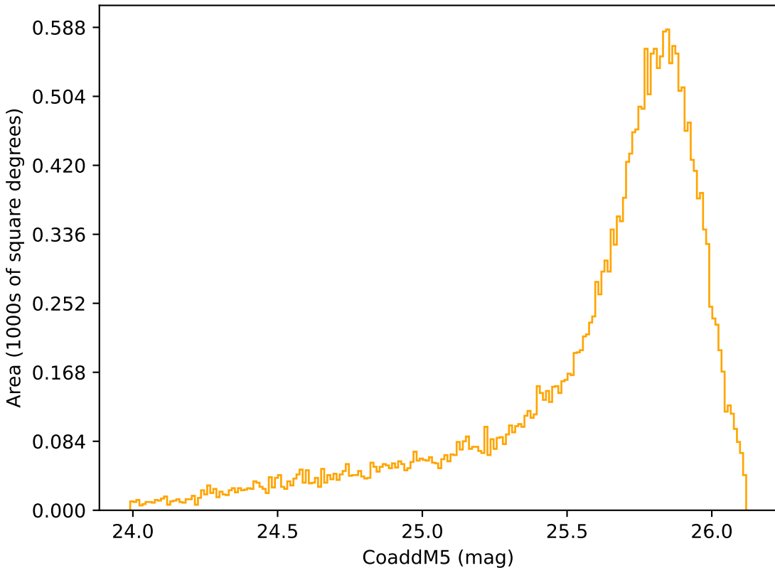
too_elab_r256_d2_gz_v3.4_10yrs Yr 1 r band: CoaddM5
