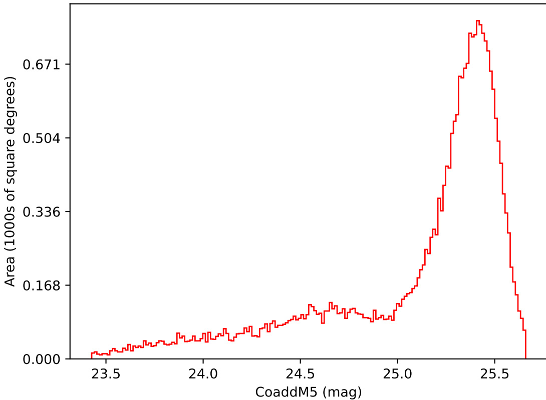
too_elab_r256_d2_gz_v3.4_10yrs Yr 1 i band: CoaddM5
