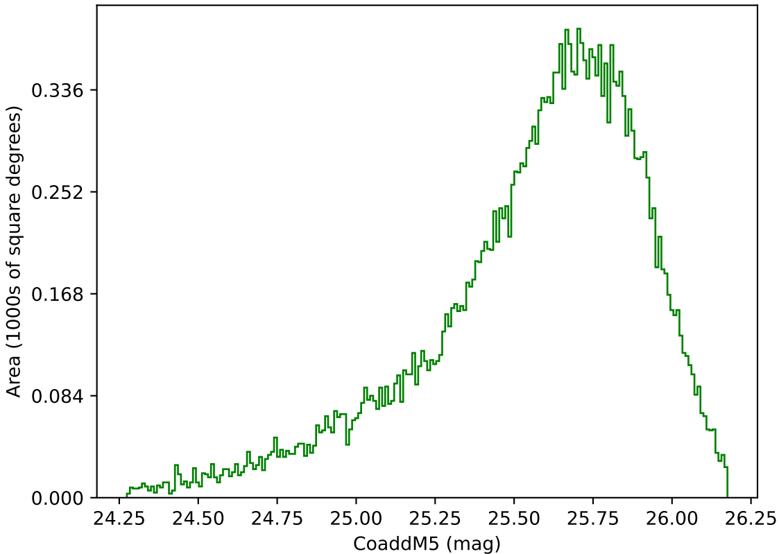
too_elab_r256_d2_gz_v3.4_10yrs Yr 1 g band: CoaddM5
