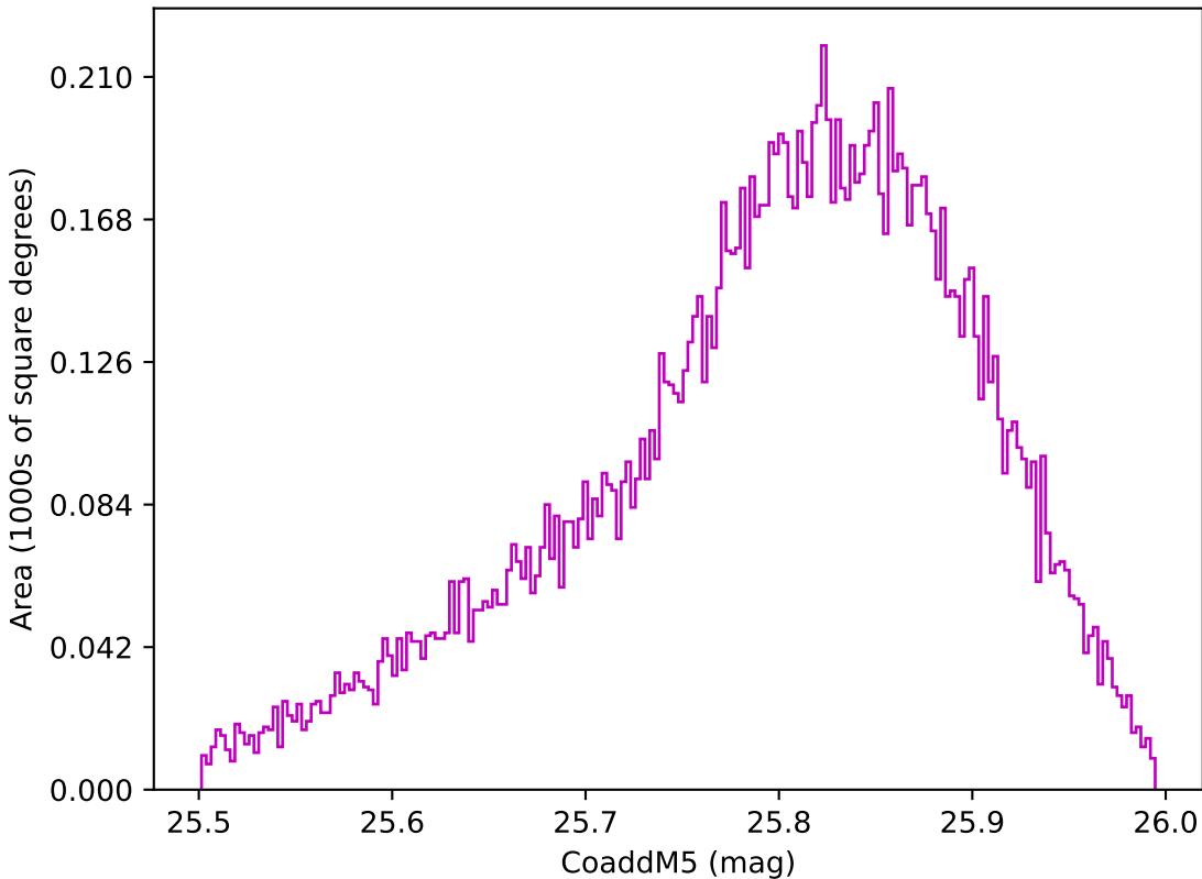
too_elab_r256_d2_gz_v3.4_10yrs WFD z band: CoaddM5
