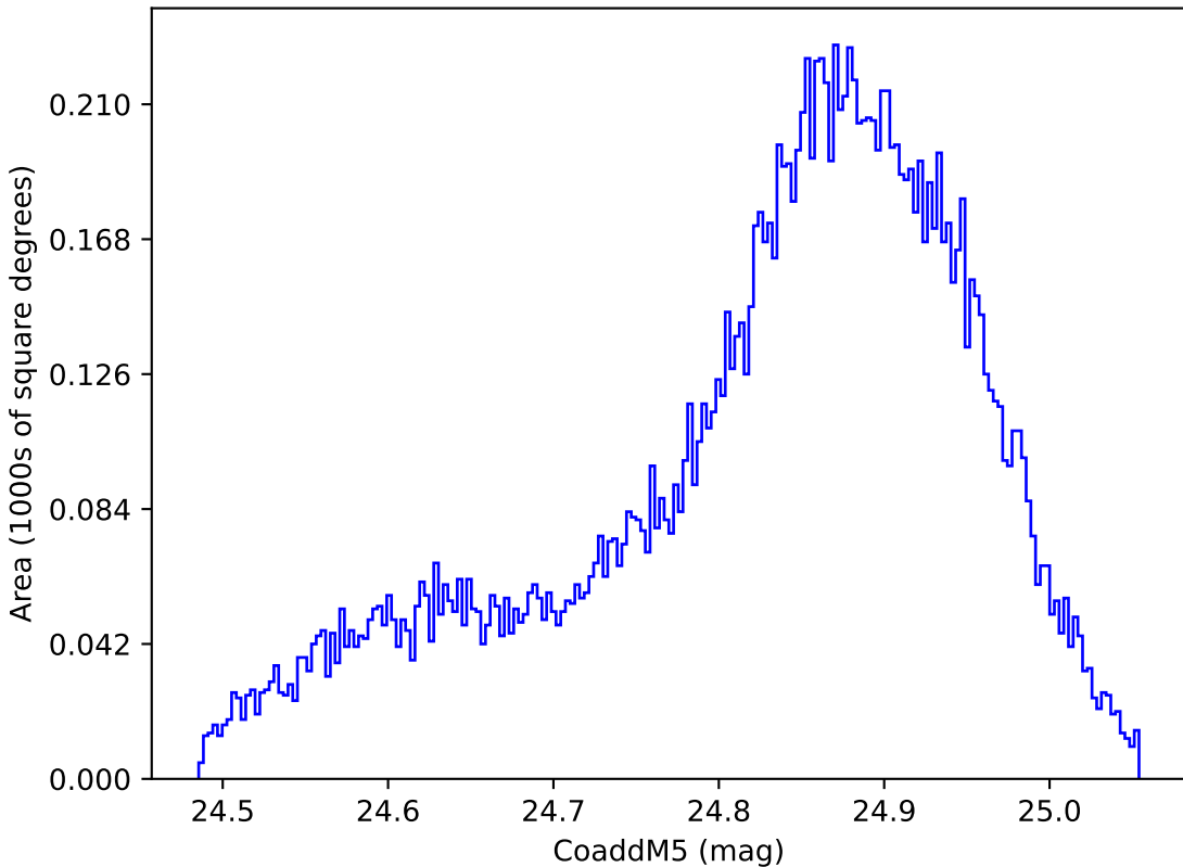
too_elab_r256_d2_gz_v3.4_10yrs WFD y band: CoaddM5
