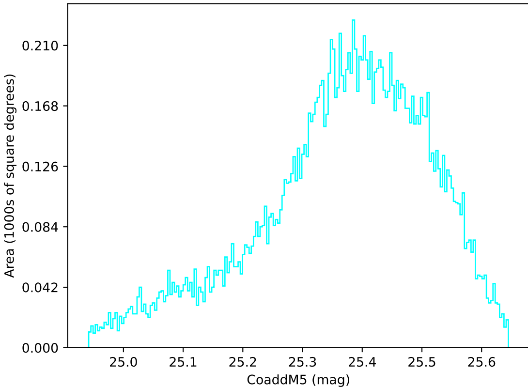
too_elab_r256_d2_gz_v3.4_10yrs WFD u band: CoaddM5
