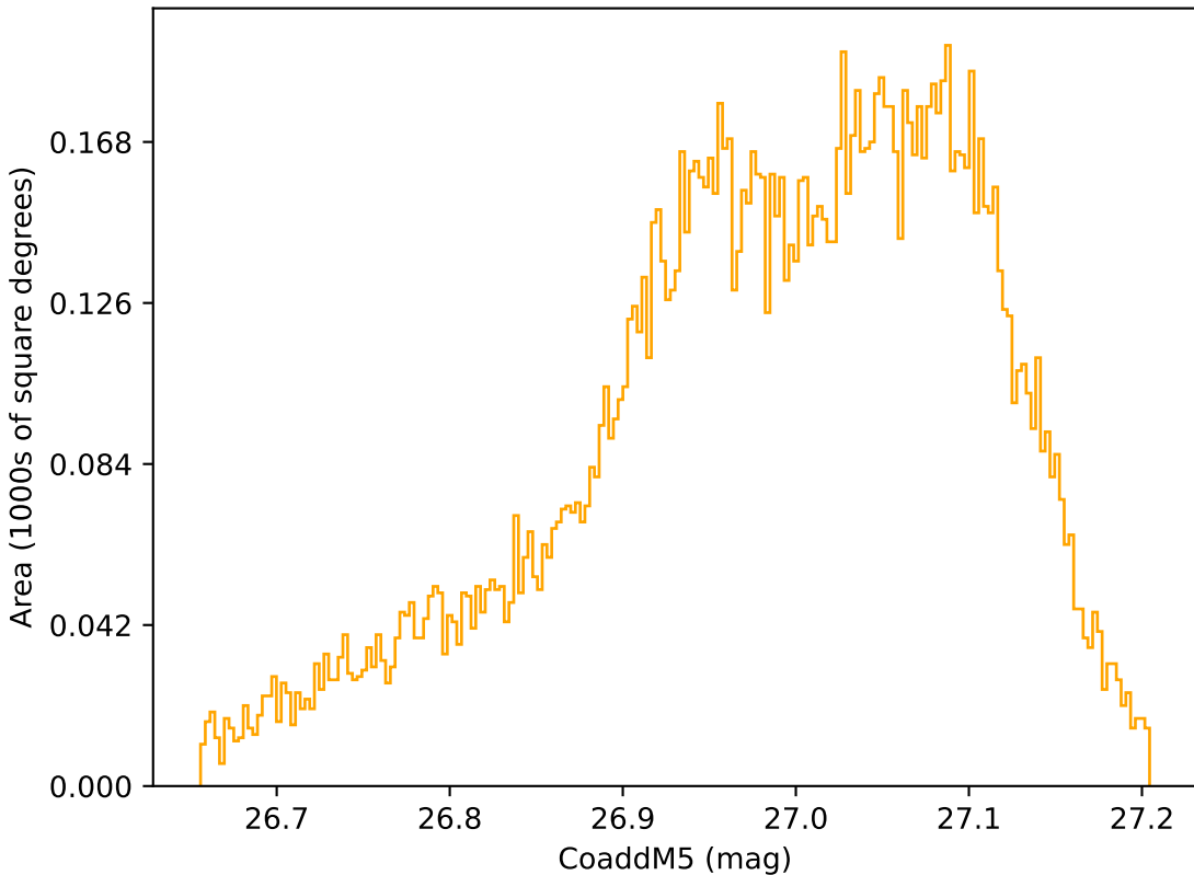
too_elab_r256_d2_gz_v3.4_10yrs WFD r band: CoaddM5
