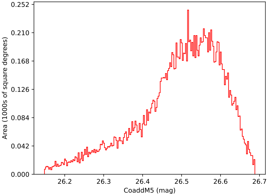
too_elab_r256_d2_gz_v3.4_10yrs WFD i band: CoaddM5
