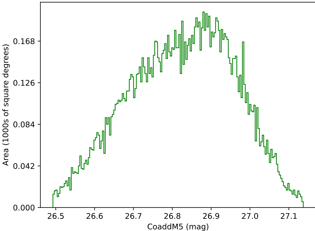
too_elab_r256_d2_gz_v3.4_10yrs WFD g band: CoaddM5
