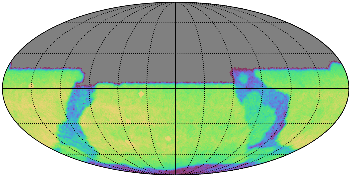
too_elab_r256_d2_gz_v3.4_10yrs All sky u band: CoaddM5
