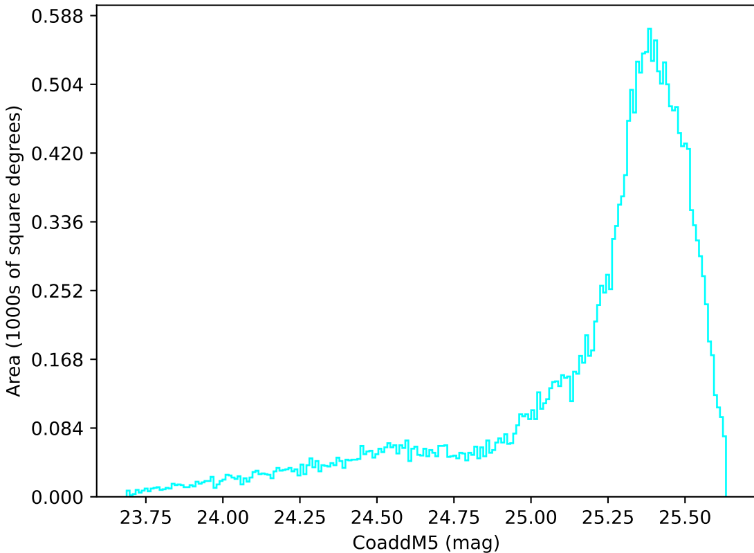
too_elab_r256_d2_gz_v3.4_10yrs All sky u band: CoaddM5
