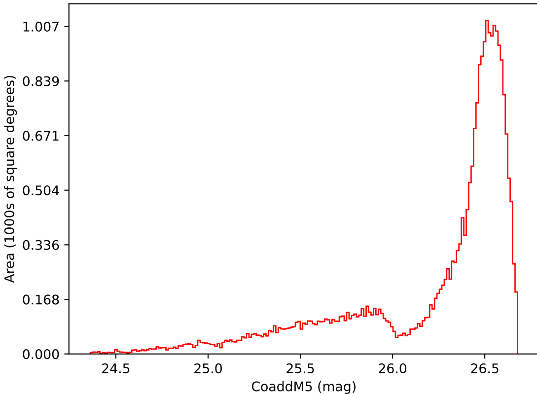
too_elab_r256_d2_gz_v3.4_10yrs All sky i band: CoaddM5
