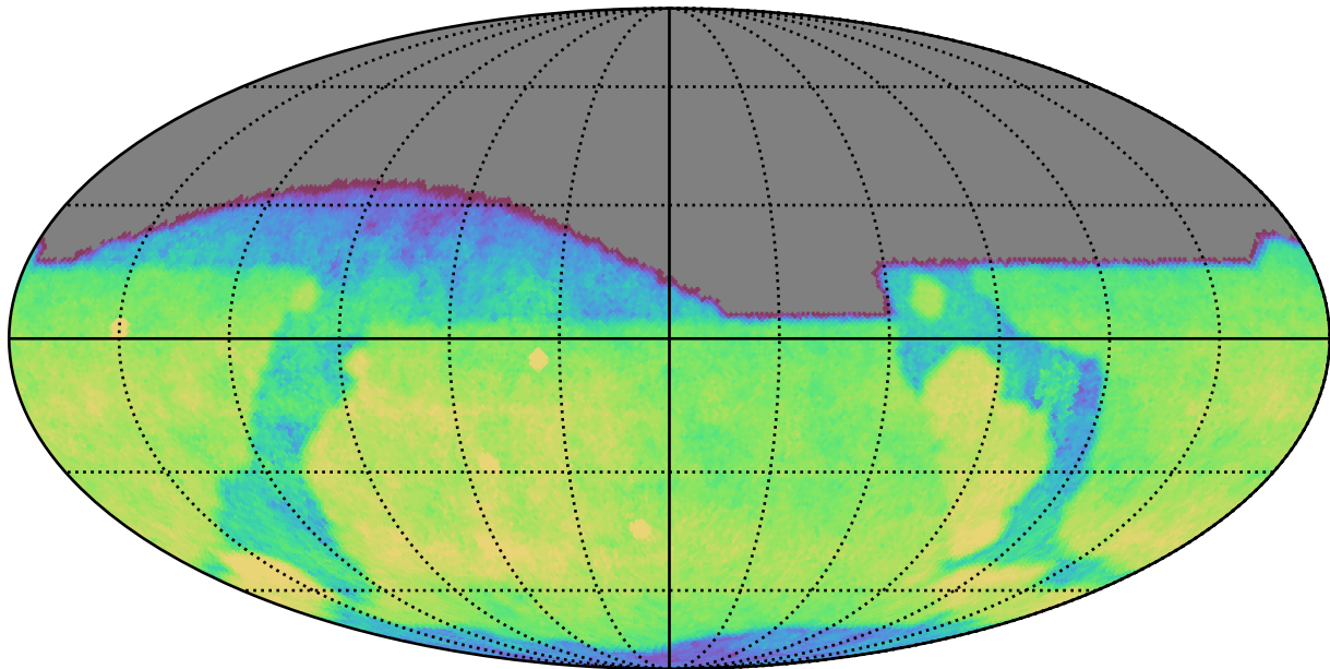
too_elab_r256_d2_gz_v3.4_10yrs All sky g band: CoaddM5
