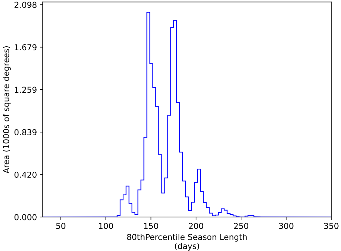
too_elab_r256_d2_gz_v3.4_10yrs WFD y band: 80thPercentile Season Length
