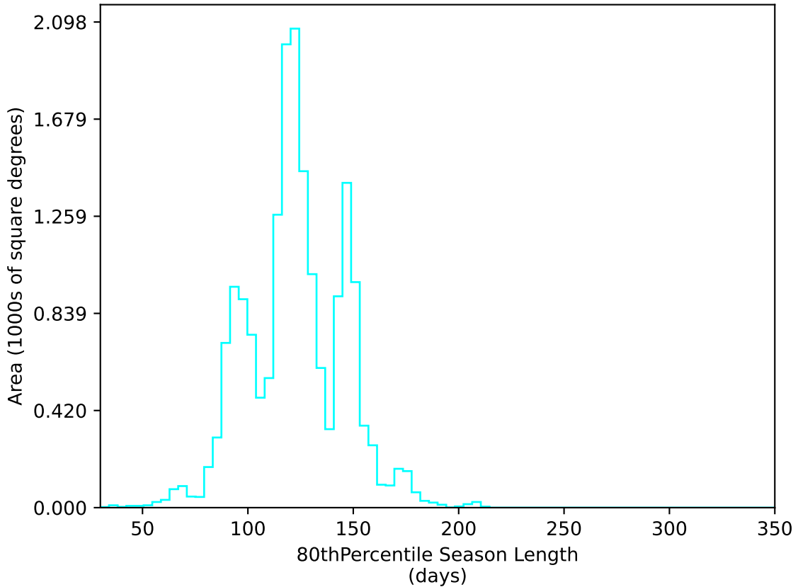
too_elab_r256_d2_gz_v3.4_10yrs WFD u band: 80thPercentile Season Length
