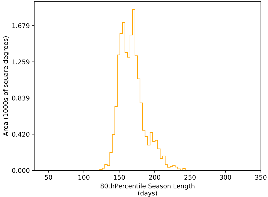
too_elab_r256_d2_gz_v3.4_10yrs WFD r band: 80thPercentile Season Length
