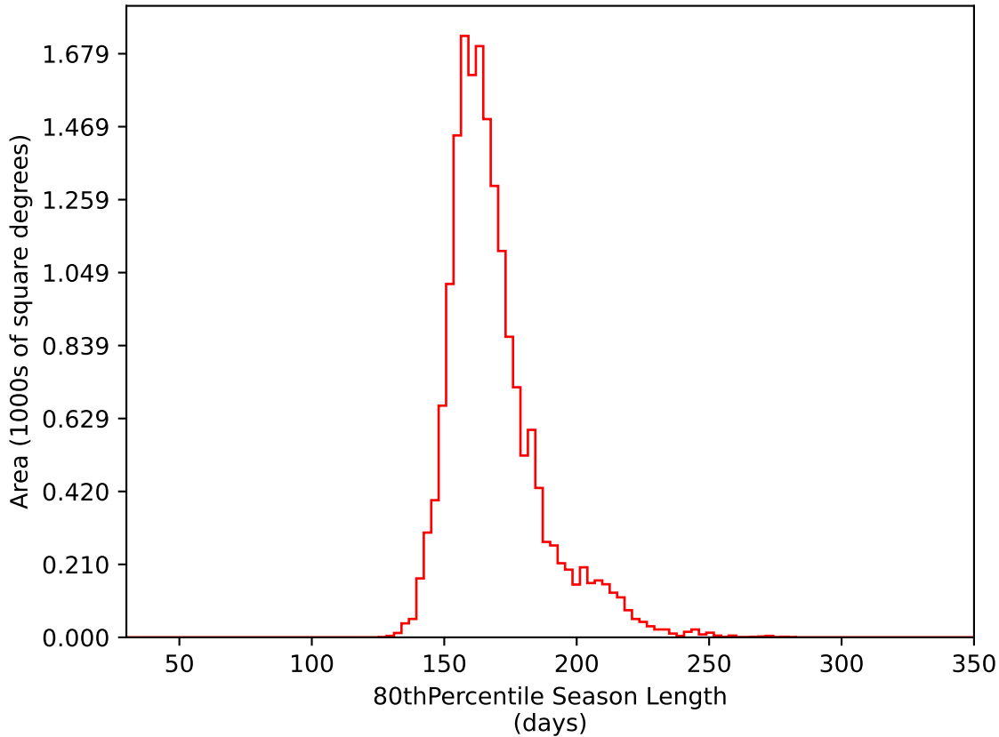
too_elab_r256_d2_gz_v3.4_10yrs WFD i band: 80thPercentile Season Length
