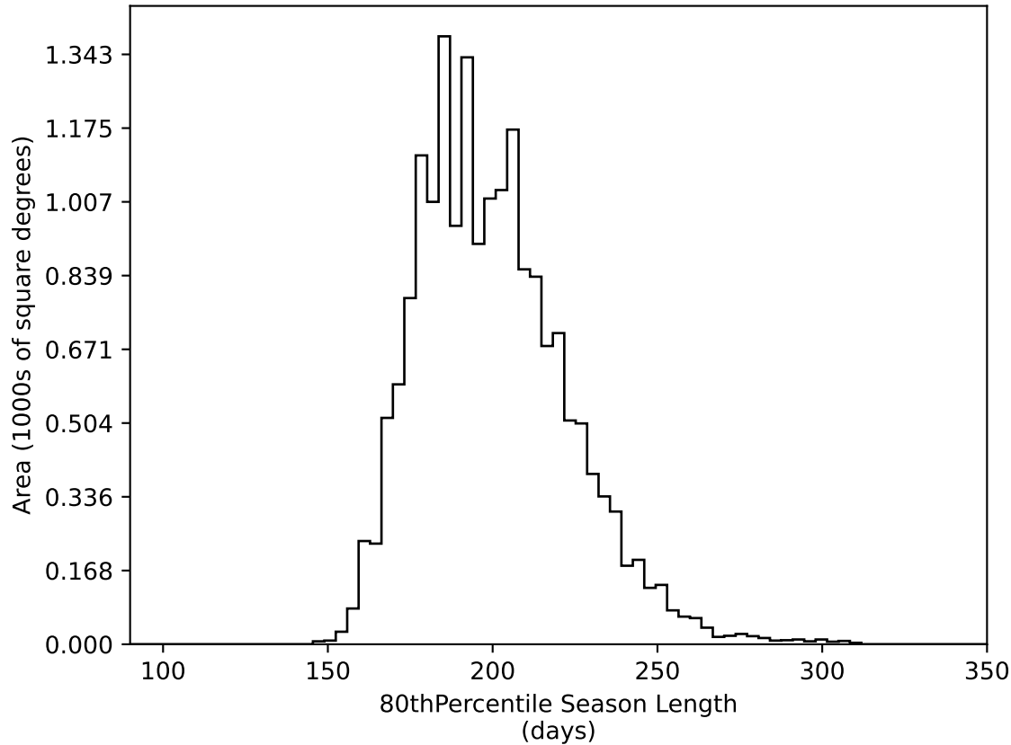
too_elab_r256_d2_gz_v3.4_10yrs WFD all bands: 80thPercentile Season Length
