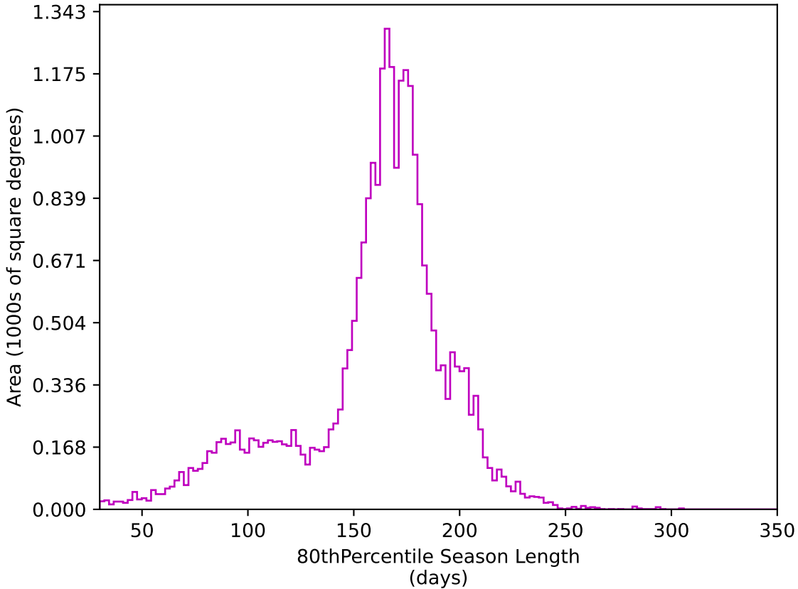
too_elab_r256_d2_gz_v3.4_10yrs All sky z band: 80thPercentile Season Length
