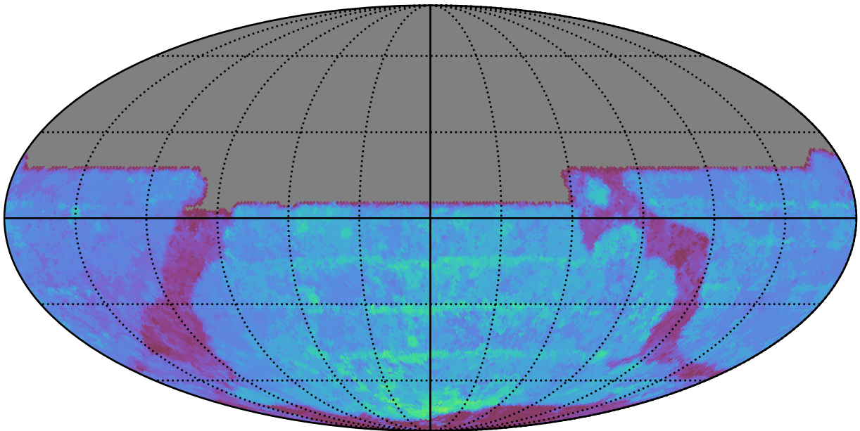
too_elab_r256_d2_gz_v3.4_10yrs All sky y band: 80thPercentile Season Length
