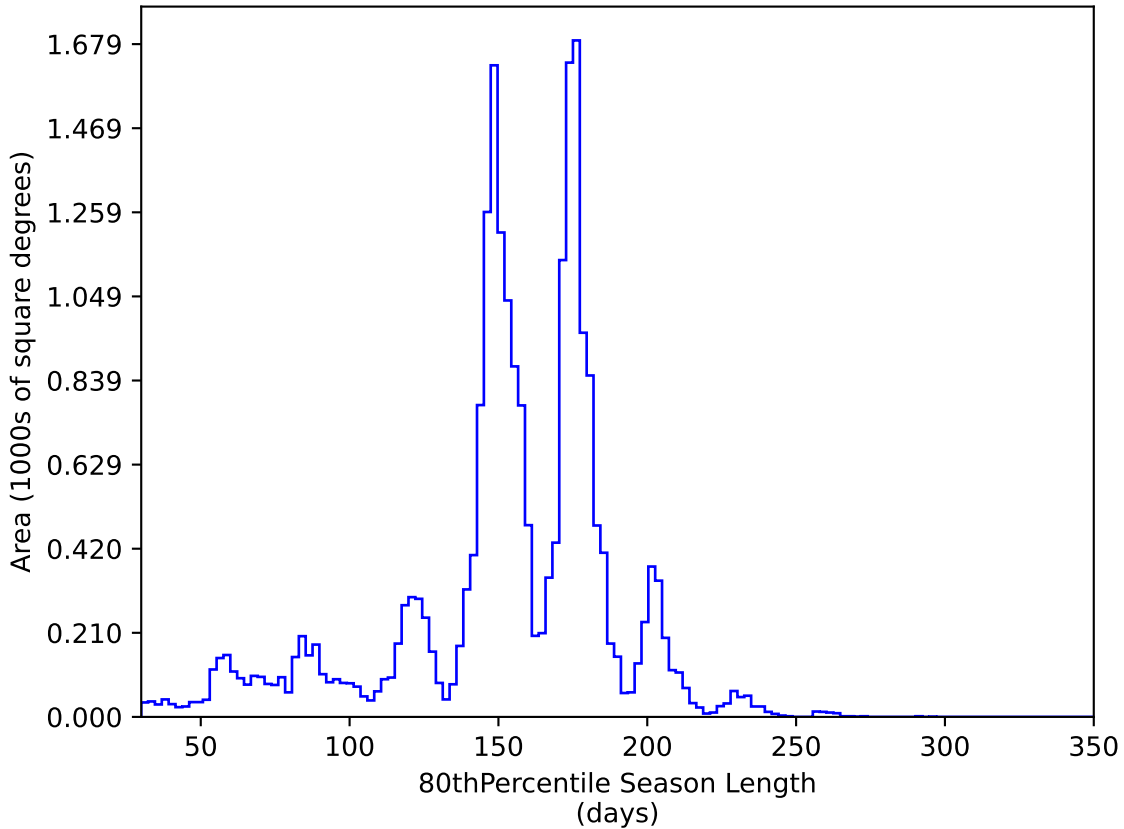
too_elab_r256_d2_gz_v3.4_10yrs All sky y band: 80thPercentile Season Length
