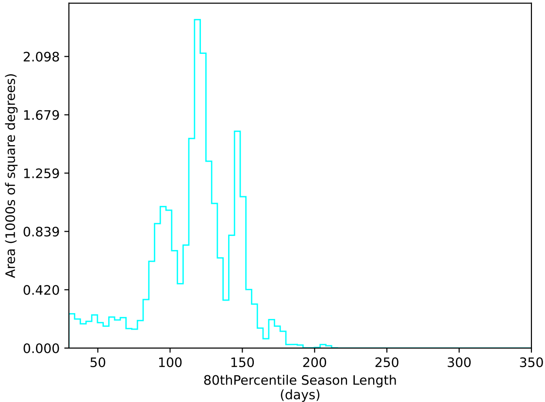
too_elab_r256_d2_gz_v3.4_10yrs All sky u band: 80thPercentile Season Length
