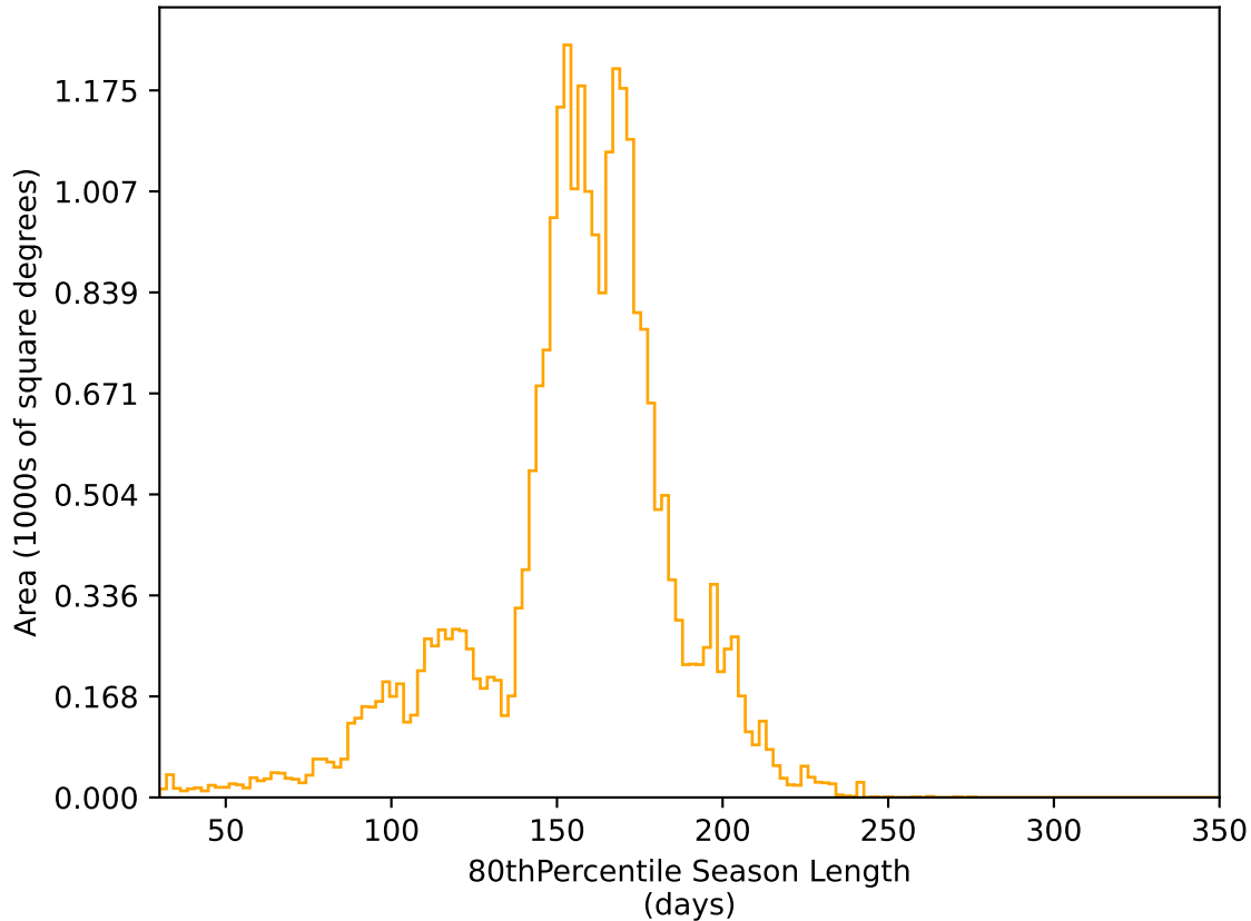
too_elab_r256_d2_gz_v3.4_10yrs All sky r band: 80thPercentile Season Length
