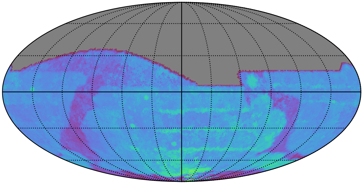
too_elab_r256_d2_gz_v3.4_10yrs All sky i band: 80thPercentile Season Length
