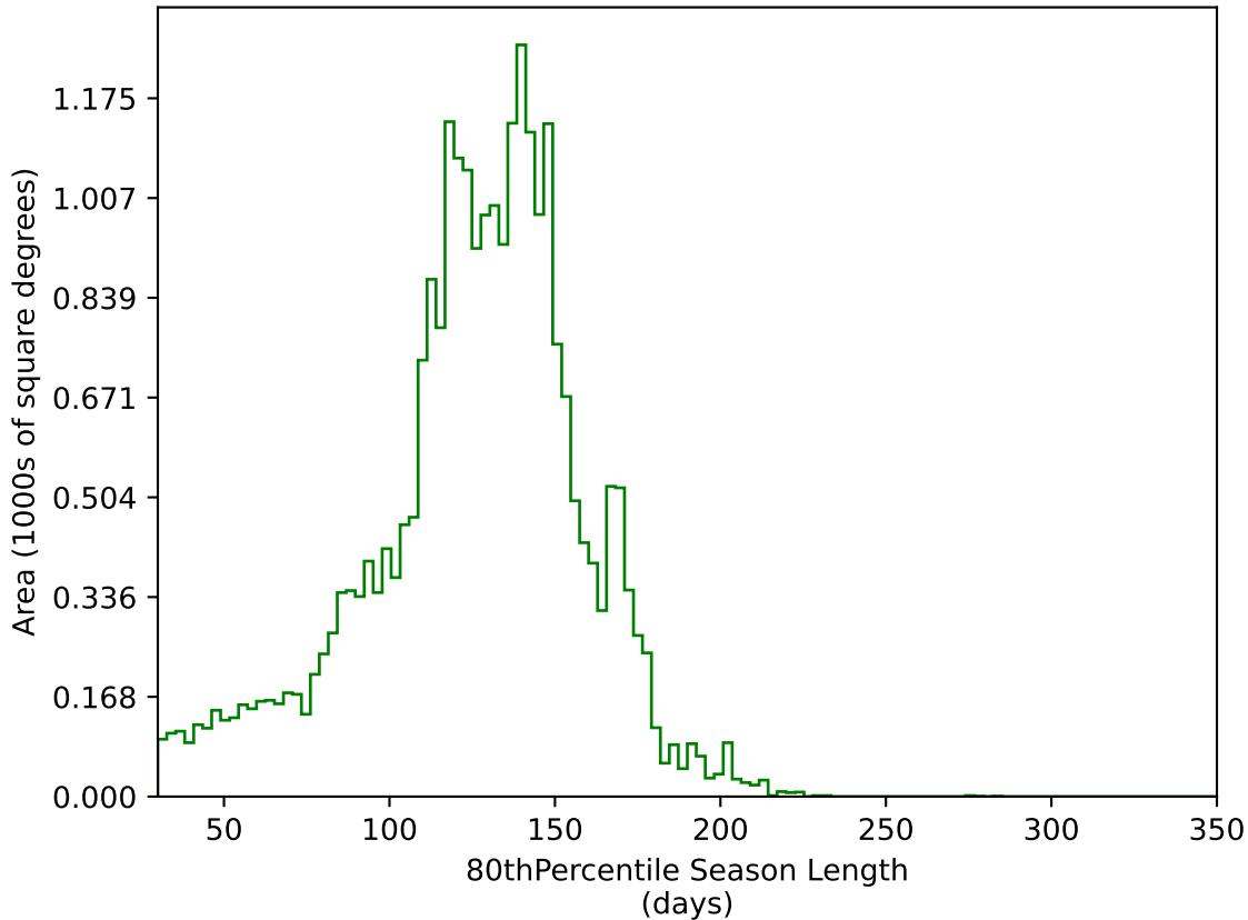
too_elab_r256_d2_gz_v3.4_10yrs All sky g band: 80thPercentile Season Length
