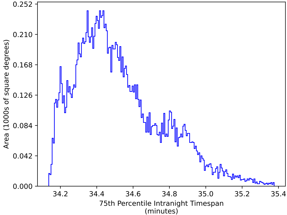
too_elab_r256_d2_gz_v3.4_10yrs WFD zy bands: 75th Percentile Intranight Timespan
