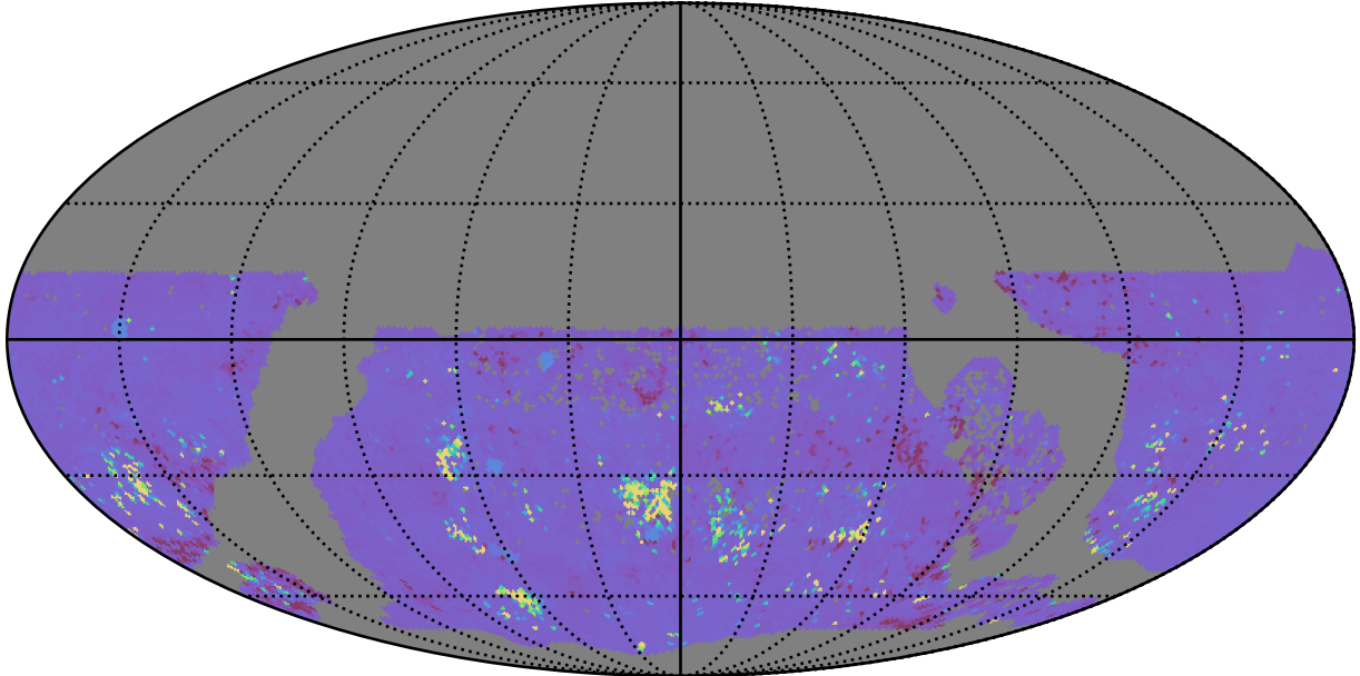
too_elab_r256_d2_gz_v3.4_10yrs WFD ug bands: 75th Percentile Intranight Timespan
