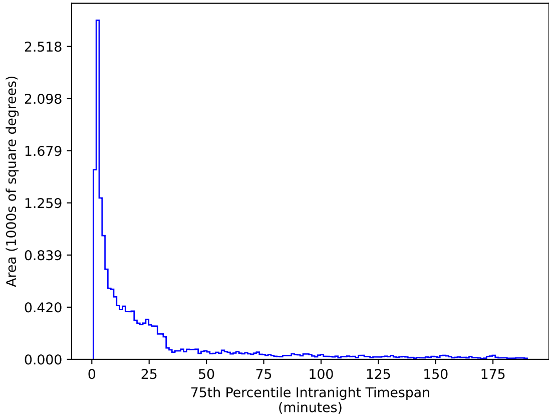
too_elab_r256_d2_gz_v3.4_10yrs WFD g band: 75th Percentile Intranight Timespan
