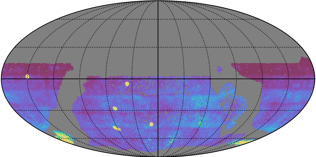
too_elab_r256_d2_gz_v3.4_10yrs WFD all bands: 75th Percentile Intranight Timespan
