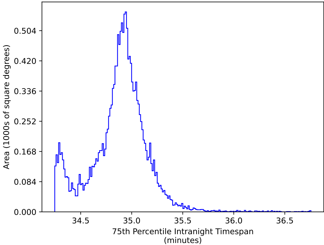
too_elab_r256_d2_gz_v3.4_10yrs WFD all bands: 75th Percentile Intranight Timespan
